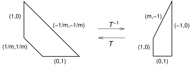
FIGURE 1. Hirzebruch surfaces.
