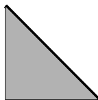
FIGURE 1. An origami polytope for a 4-sphere
