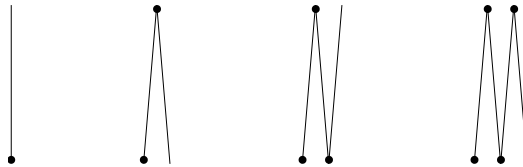
FIGURE 12. Toric origami real projective planes
