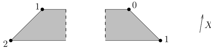
FIGURE 18. The unfolded set \mathcal{P}^u for a toric manifold with a flag-like moment polytope
