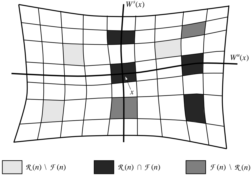
FIGURE 1. The procedure of “filling in” rectangles.
