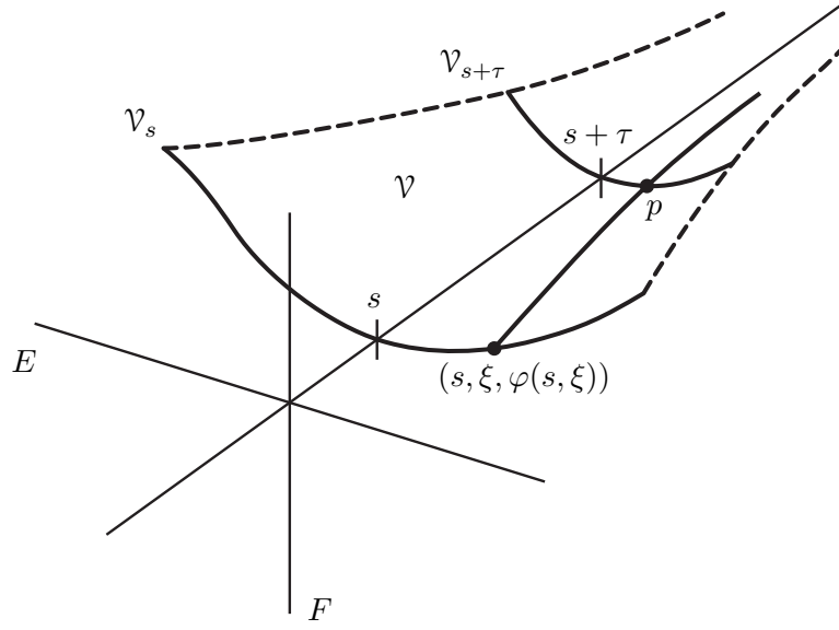
FIGURE 1. A stable manifold \mathcal{V} of the origin. In order that \mathcal{V} is invariant under the flow \Psi_\tau we require that p = \Psi_\tau(s, \xi, \varphi(s, \xi)) . Here the subspaces E = E(t) and F = F(t) are assumed to be independent of t .
