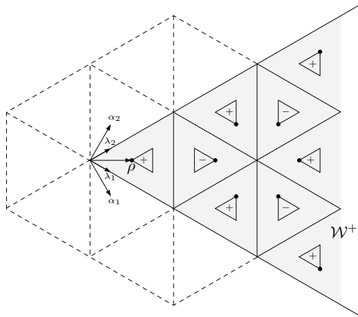
The points \lambda + \rho \in [\gamma + \rho]_k \cap \Lambda_W^+ , in the case SU(3) , k = 1 , \gamma = 0 , together with the corresponding sign \epsilon_{\lambda}
