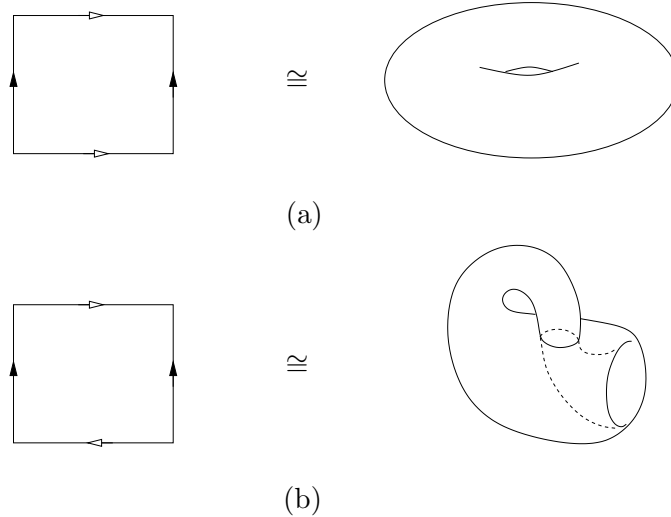
FIGURE 2. (a) Torus ( T^2 ), (b) Klein bottle ( K^2 ).
