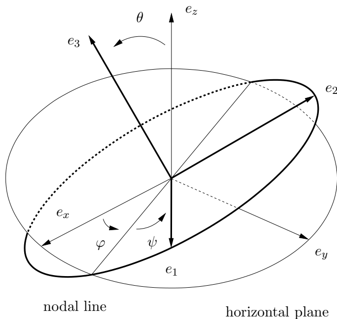
FIGURE 2. Euler angles.
