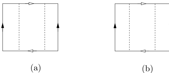
FIGURE 6. (a) Klein bottle, (b) Real projective plane.
