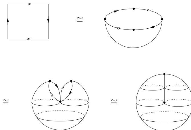
FIGURE 3. Real projective plane ( \mathbb{R}P^2 ).
