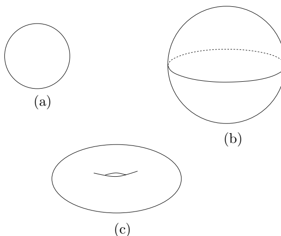
FIGURE 1. (a) S^1 , (b) S^2 , (c) Torus of revolution.
