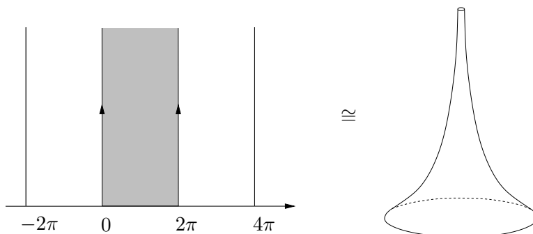
FIGURE 3. Pseudosphere.
