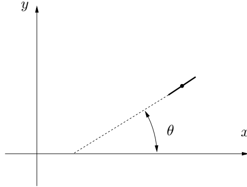
FIGURE 4. Ice skate.
